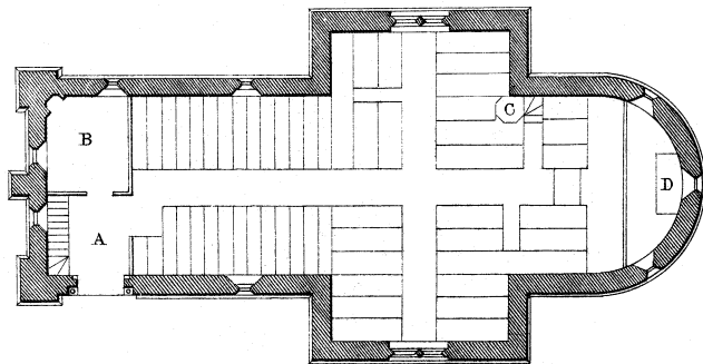
P L A N .
